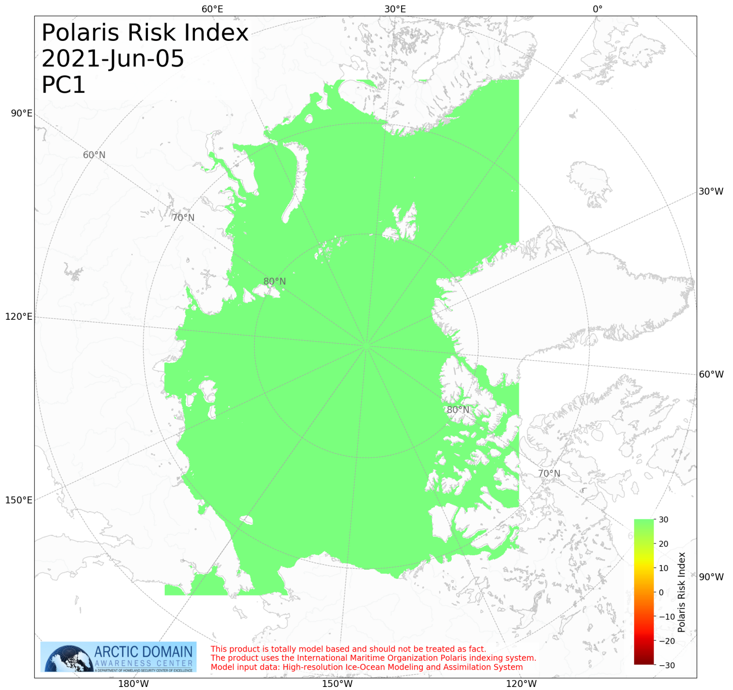
Figure 2: Risk Index pc1 for Day 1
