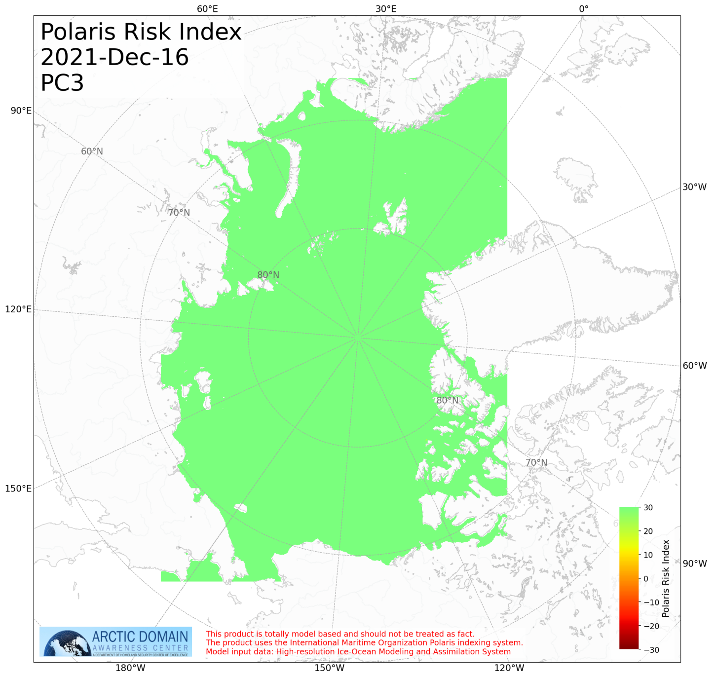
Figure 7: Risk Index pc3 for Day 6
