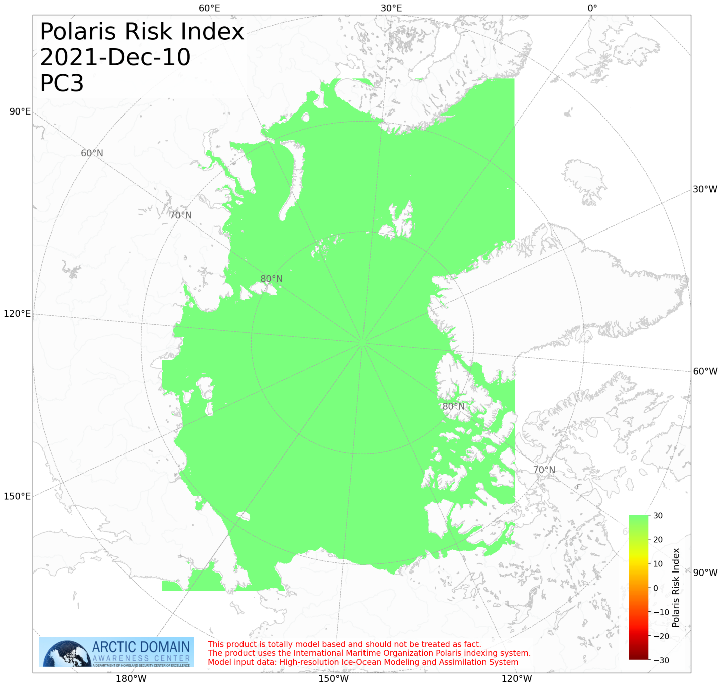
Figure 1: Risk Index pc3 for Day 0
