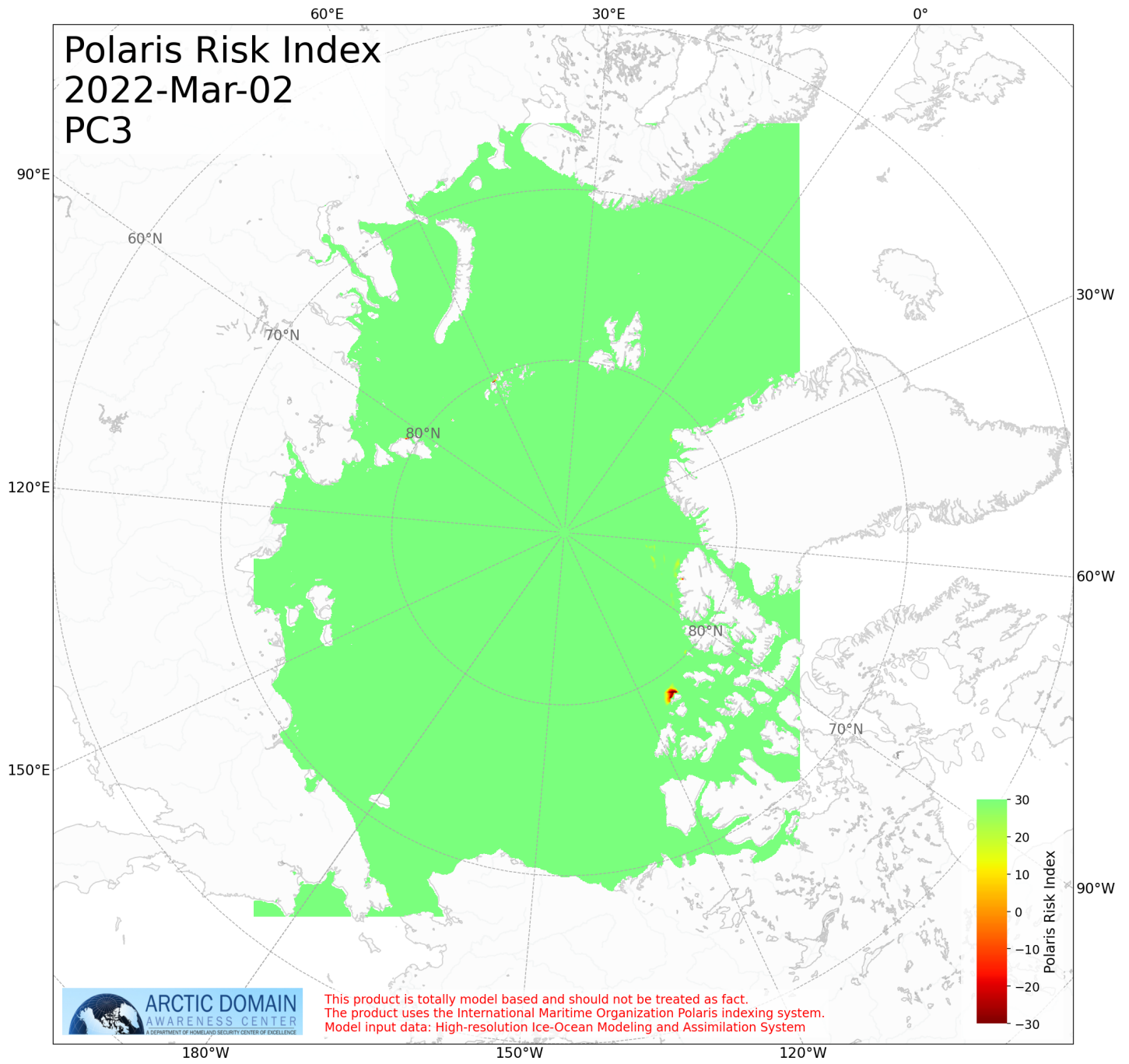
Figure 12: Risk Index pc3 for Day 11
