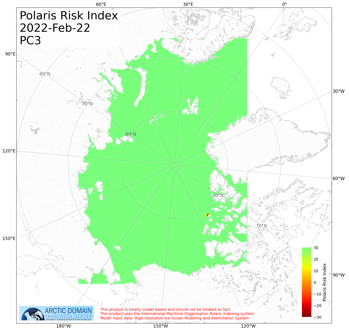
Figure 4: Risk Index pc3 for Day 3
