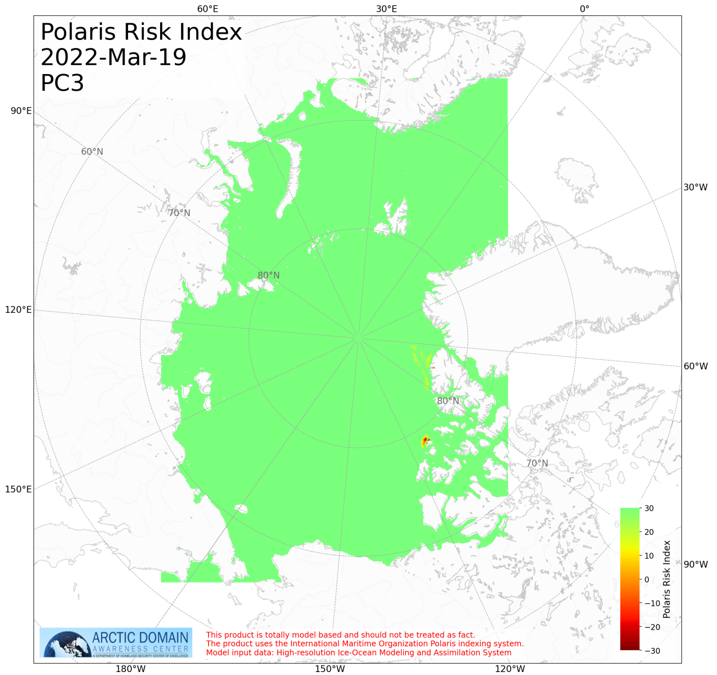
Figure 17: Risk Index pc3 for Day 28
