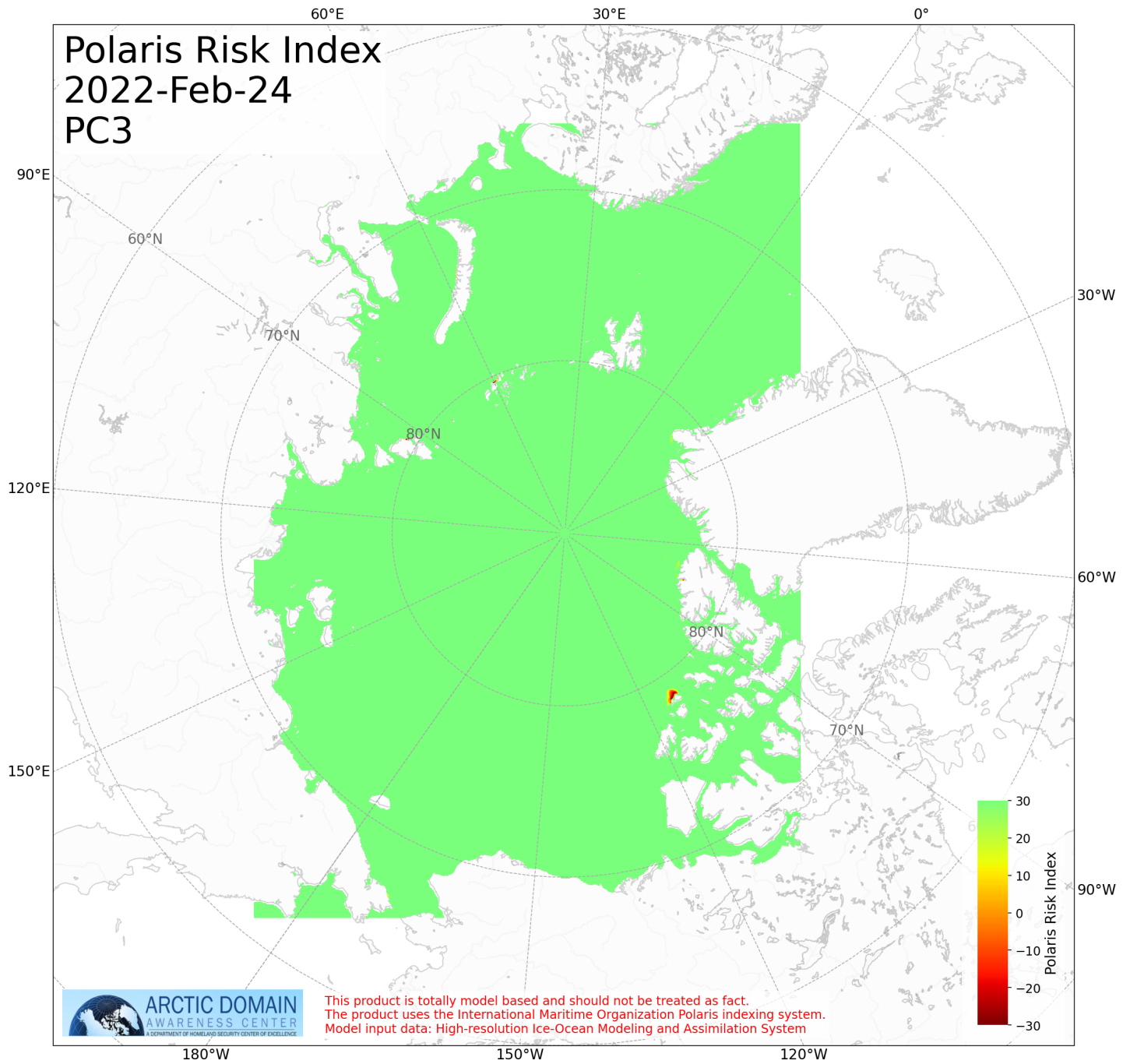
Figure 6: Risk Index pc3 for Day 5
