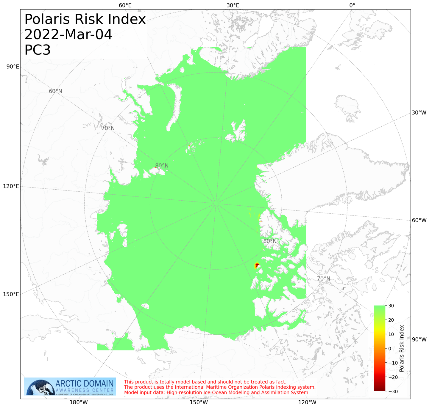
Figure 14: Risk Index pc3 for Day 13
