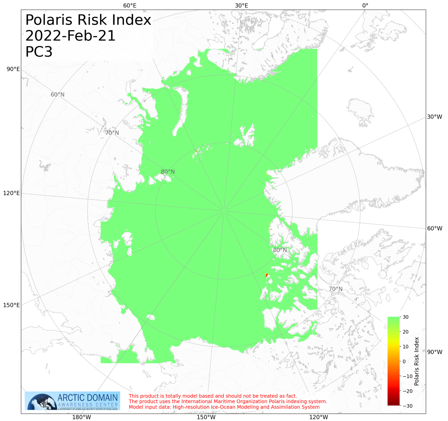
Figure 3: Risk Index pc3 for Day 2
