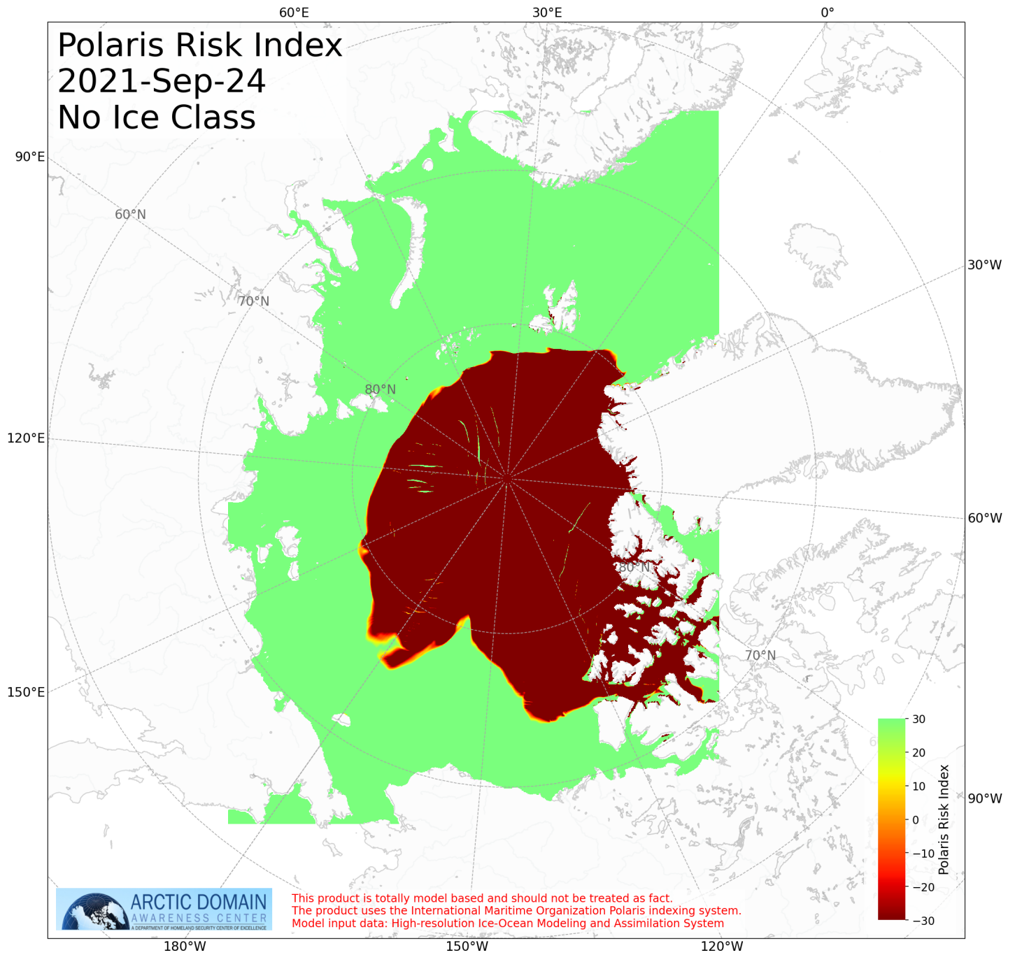
Figure 15: Risk Index no-class for Day 14
