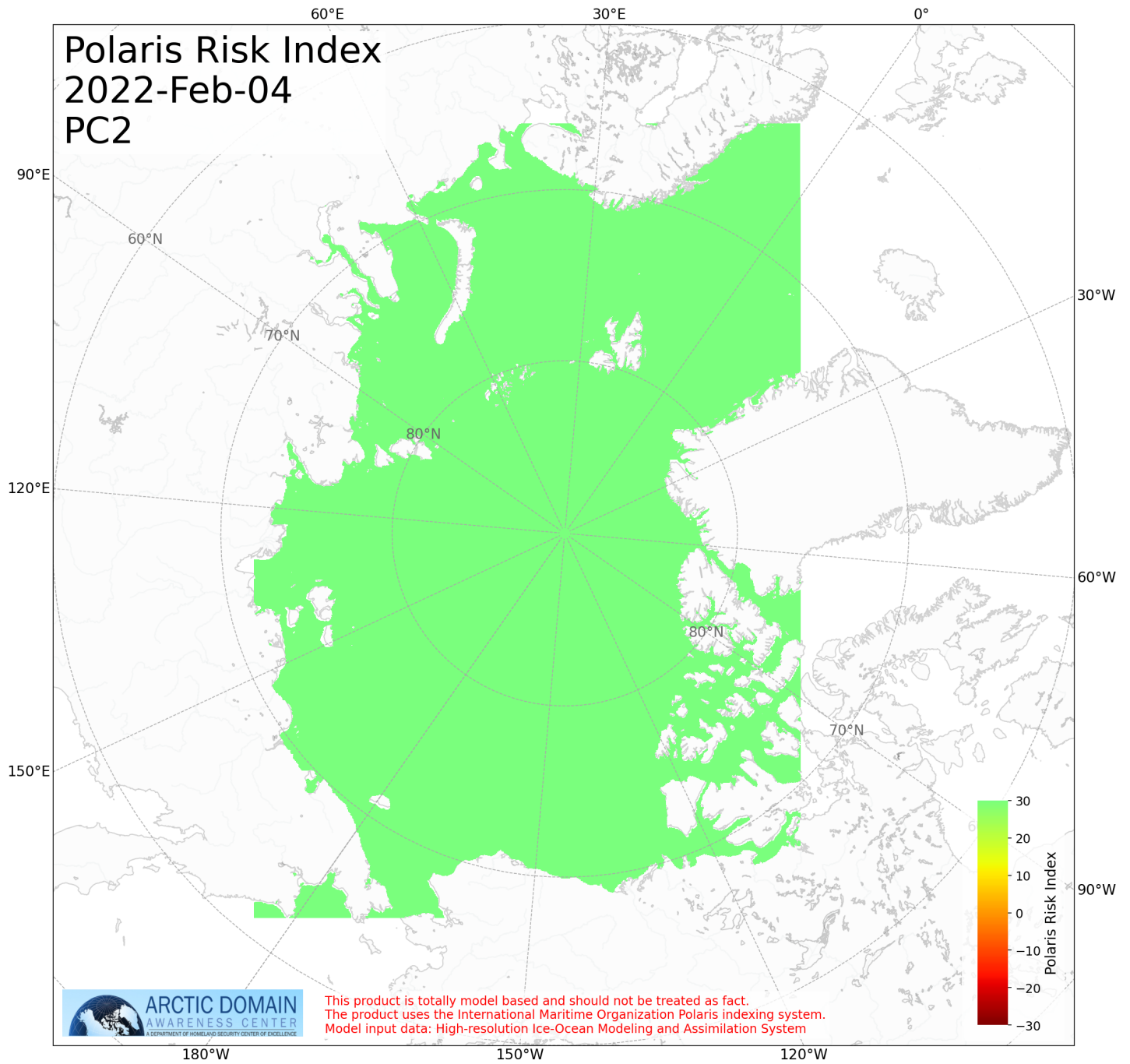
Figure 14: Risk Index pc2 for Day 13
