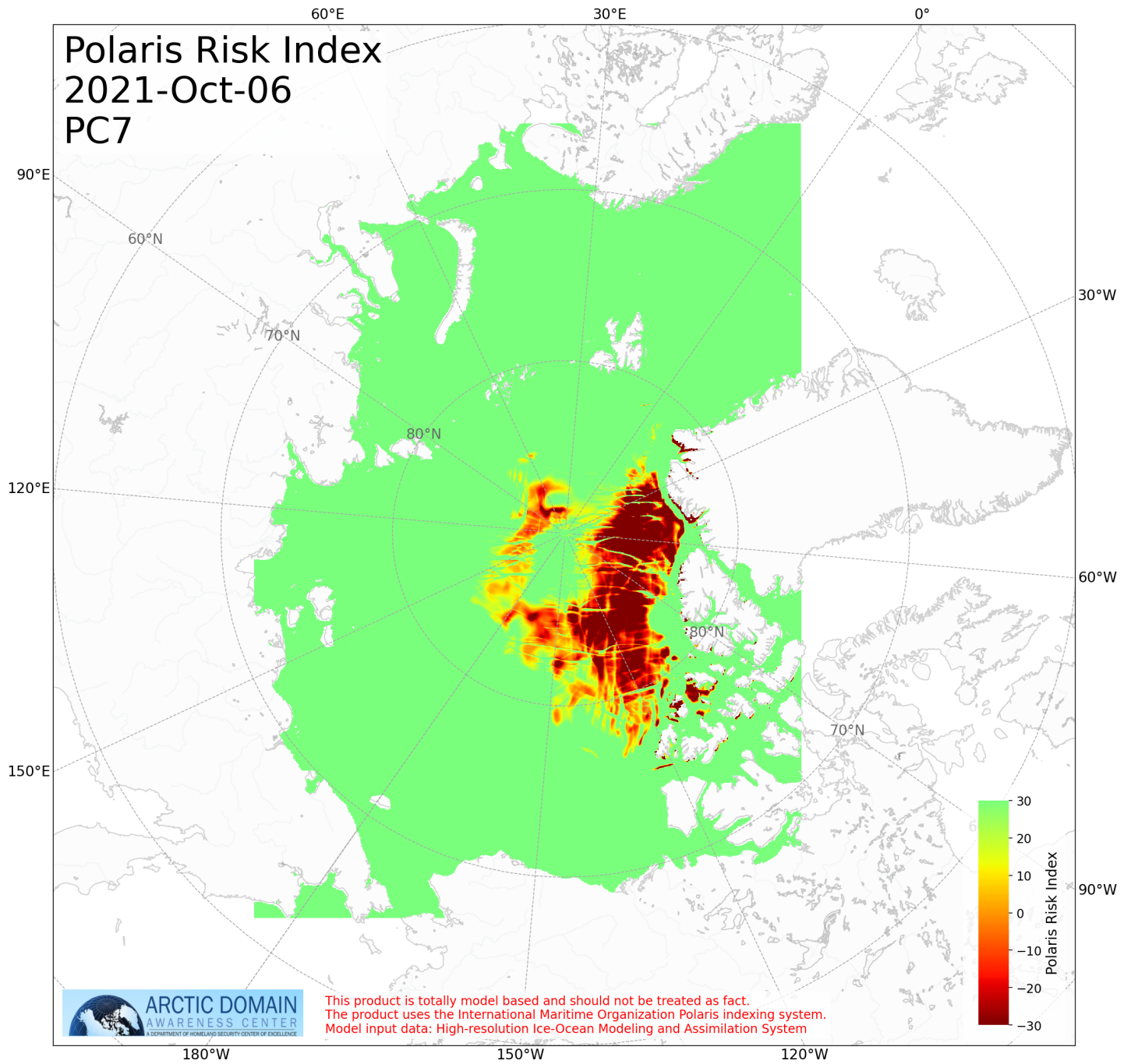
Figure 6: Risk Index pc7 for Day 5
